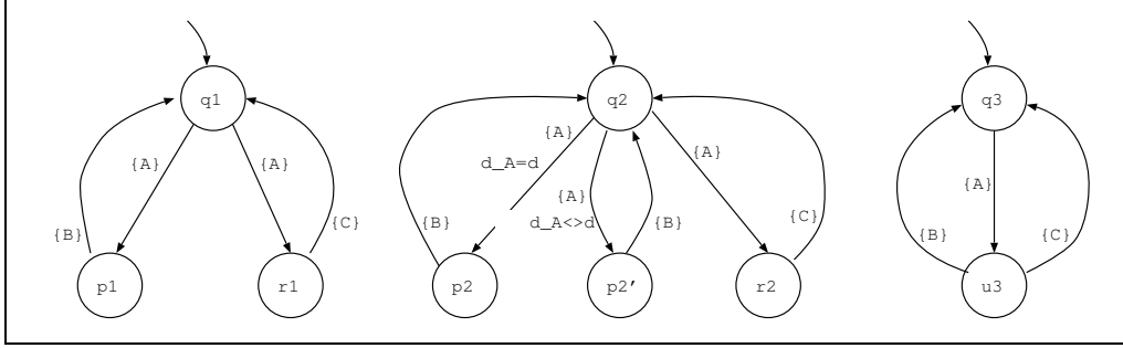
Fig. 19. Similarity and bisimilarity
