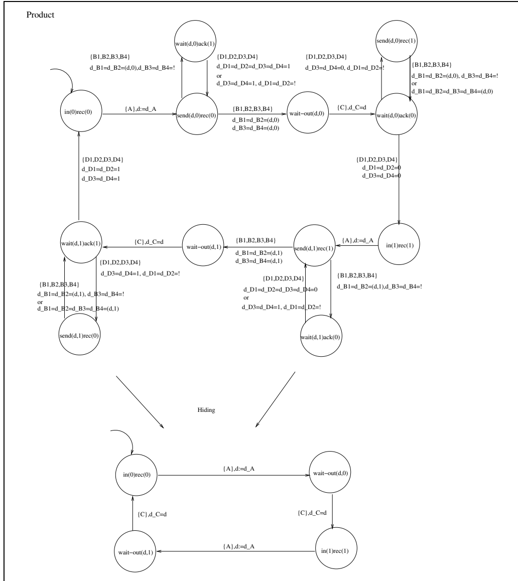
Fig. 23. ABP: Product of automata
