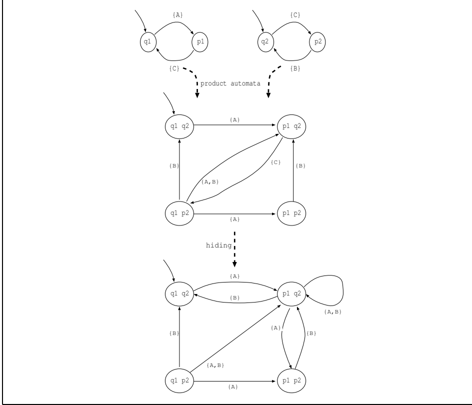
Fig. 10. Composition of two FIFO1 channels
