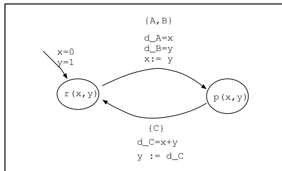
Fig. 16. Parameterized constraint automaton for Fibonacci series
