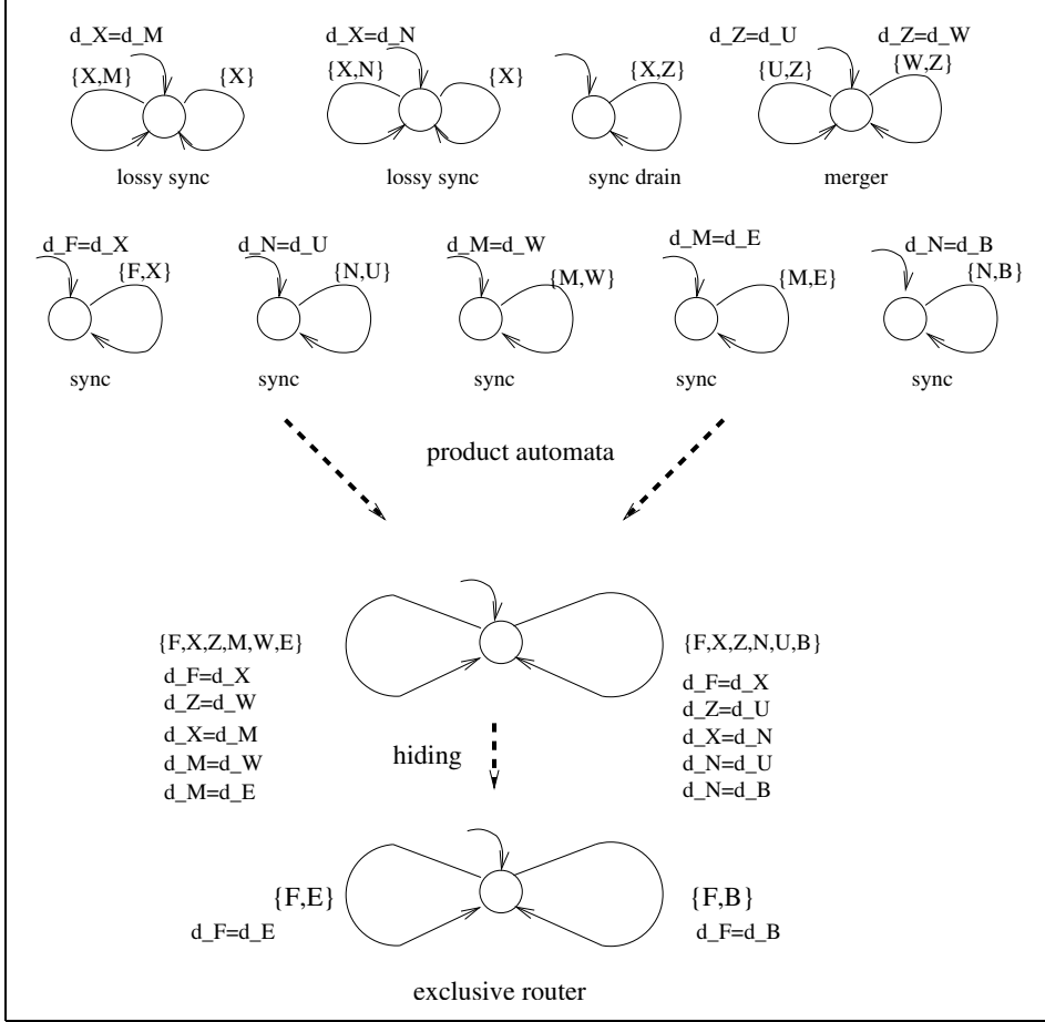
Fig. 11. Exclusive router obtained through composition of basic Reo channels
