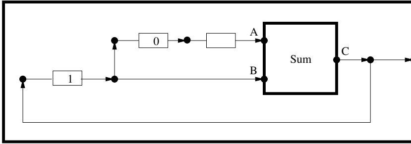
Fig. 14. Reo circuit for Fibonacci series
