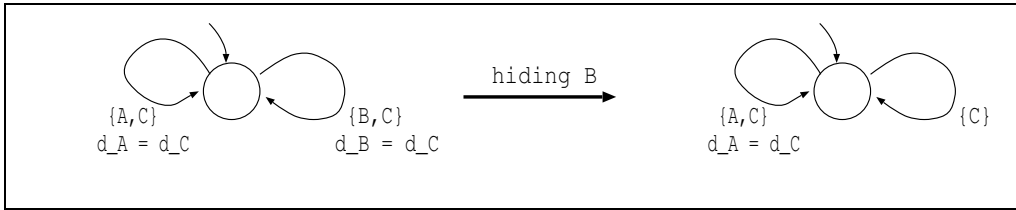
Fig. 9. Hiding a node of the merger
