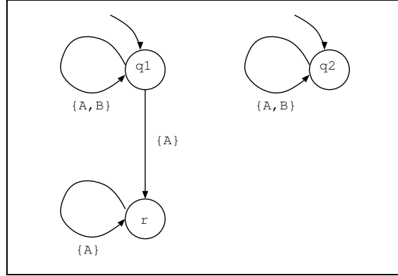
Fig. 20. Language equivalence and bisimilarity
