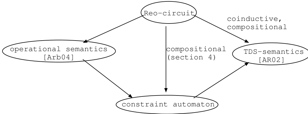
Fig. 18. Relationships among various semantics for Reo
