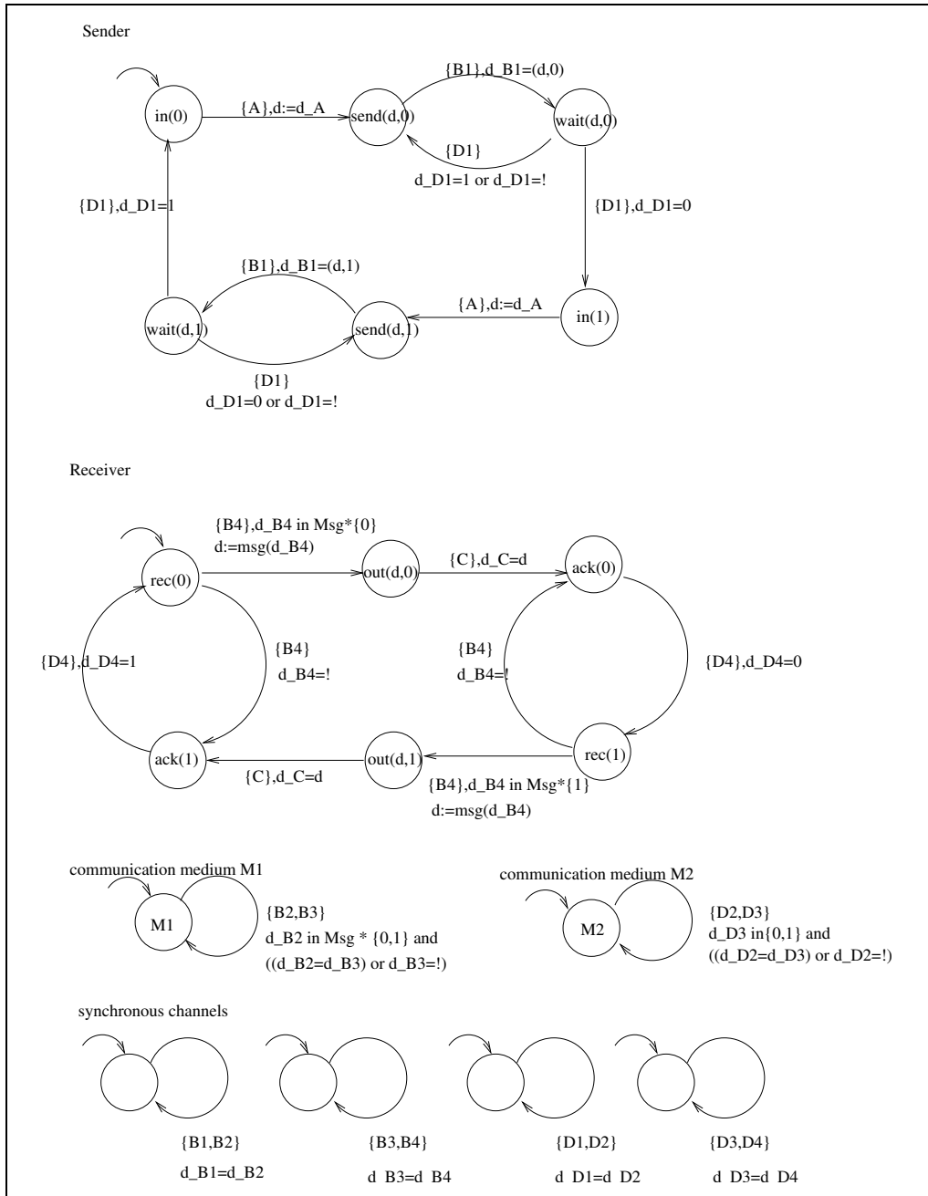
Fig. 22. ABP: Constraint automata of Components
