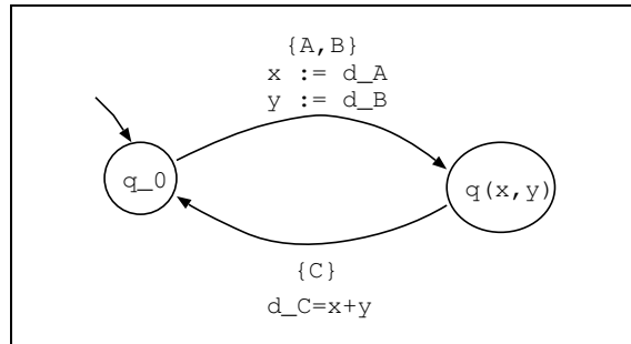
Fig. 15. Parameterized constraint automaton for Sum
