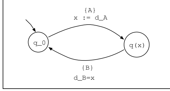
Fig. 13. Parameterized constraint automaton for a 1-bounded FIFO channel
