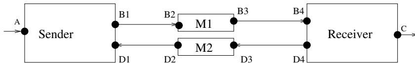
Fig. 21. ABP: Components involved
