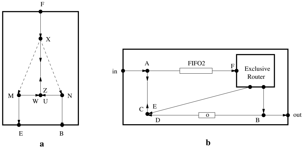
Fig. 6. Exclusive router and shift-lossy FIFO1
