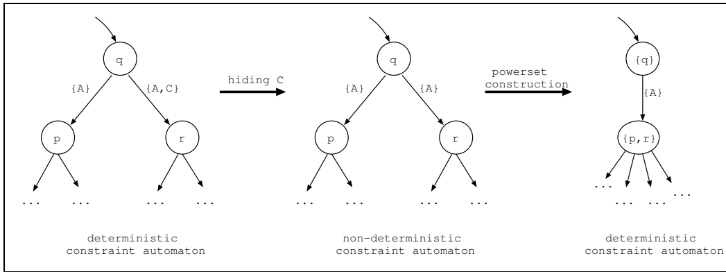
Fig. 17. Transformation of deterministic and nondeterministic constraint automata
