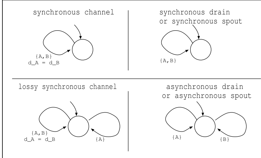
Fig. 7. Deterministic constraint automata for some basic connectors
