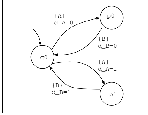
Fig. 1. Constraint automaton for a 1-bounded FIFO channel
