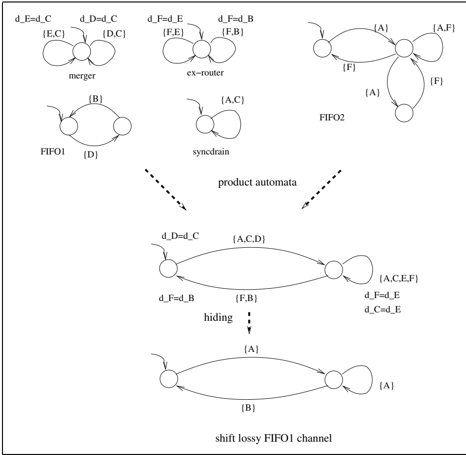
Fig. 12. Shift-lossy FIFO1 channel obtained through composition of other Reo channels
