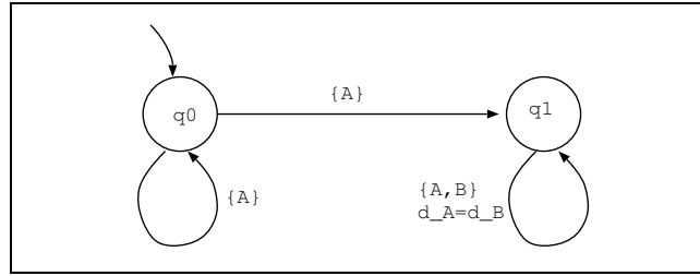
Fig. 2. A nondeterministic constraint automaton
