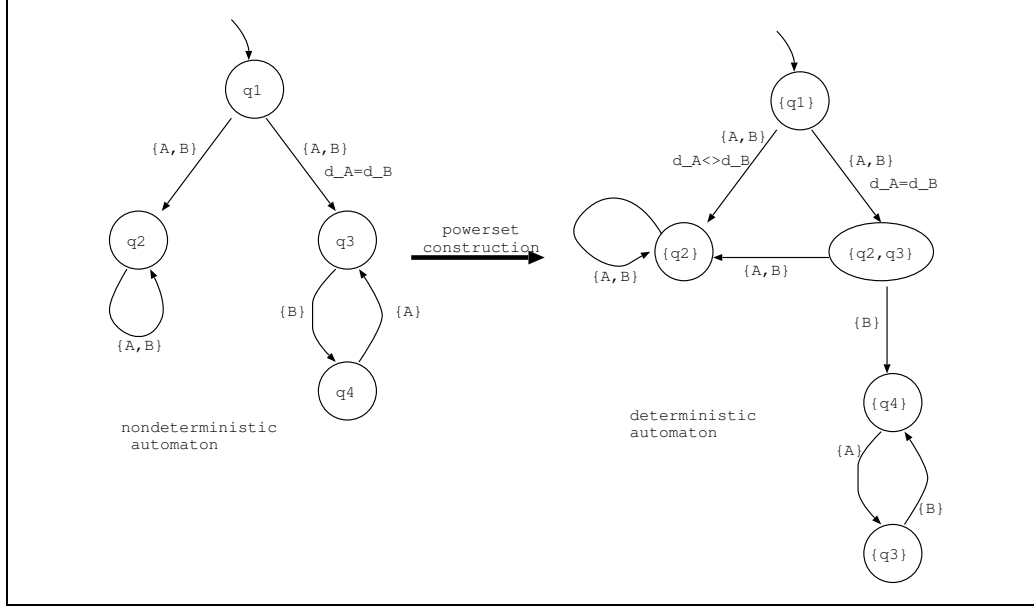
Fig. 3. Example for the powerset construction
