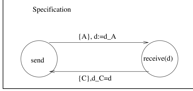
Fig. 24. ABP: Specification of the protocol
