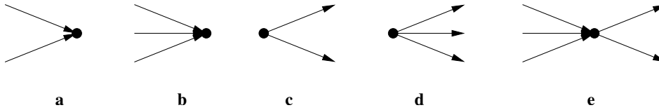
Fig. 5. Nodes in Reo
