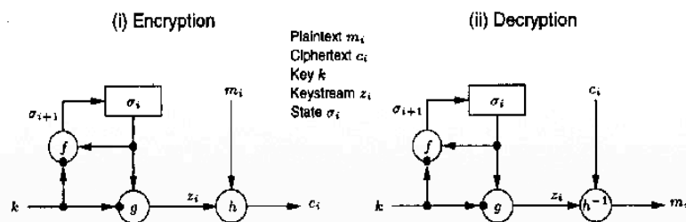
Figure 6.1: General model of a synchronous stream cipher.
