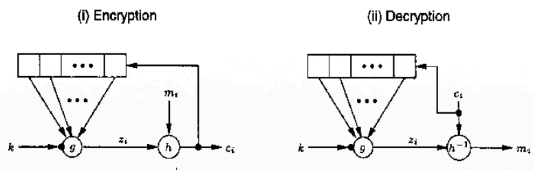
Figure 6.3: General model of a self-synchronizing stream cipher.
