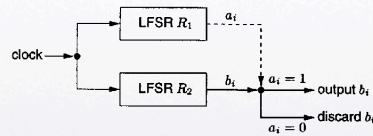
Figure 6.13: The shrinking generator.
