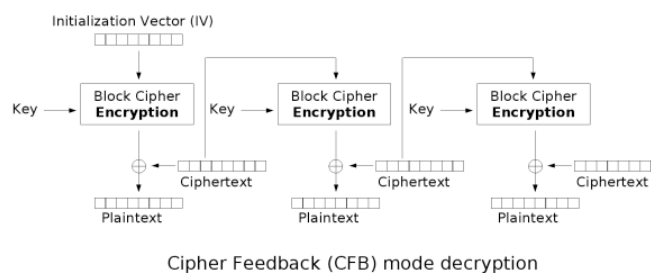
Cipher Feedback (CFB) mode decryption
