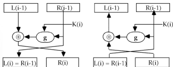
Fig 2.4 - A Round of a Feistel Cipher
