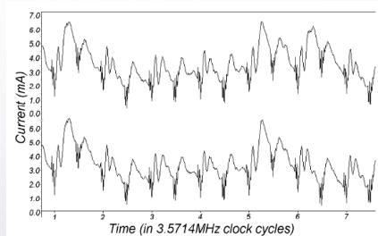
Figure 3: SPA trace showing individual clock cycles.
