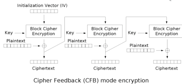
Cipher Feedback (CFB) mode encryption
