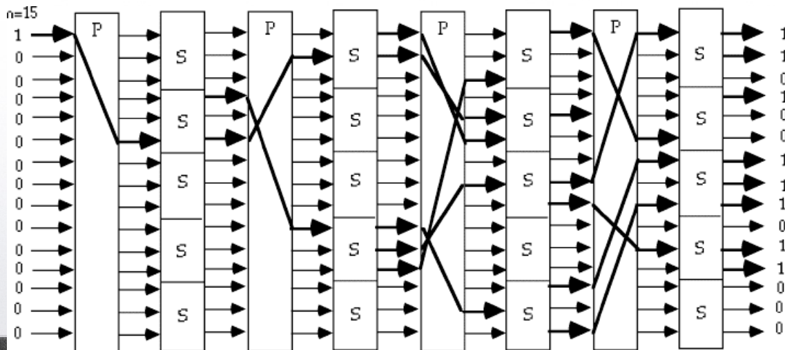
Fig 2.3 - Substitution-Permutation Network, with the Avalanche Characteristic
