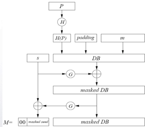
Figure 1: OAEP encoding function.
