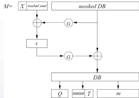
Figure 2: OAEP decoding function.
