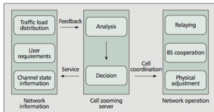
Figura 2.7: Framework do cell zooming . Source: [14].
