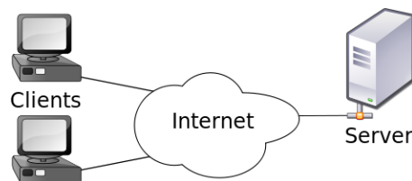
Figure 3 - Client-Server Architecture
