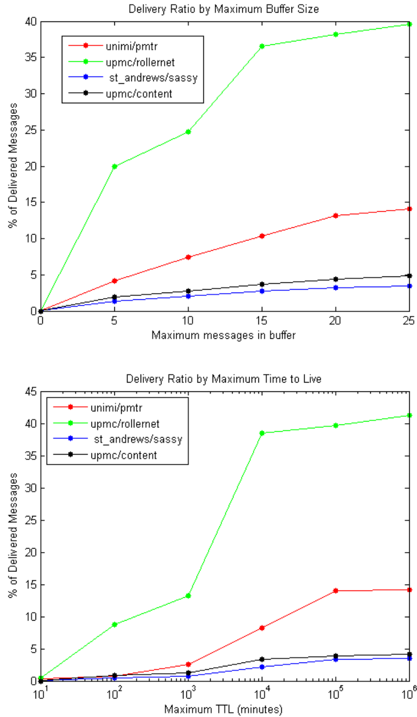
Figure 4.4: Delivery ratio with restrictions on buffer size and time to live (ONE simulation).
