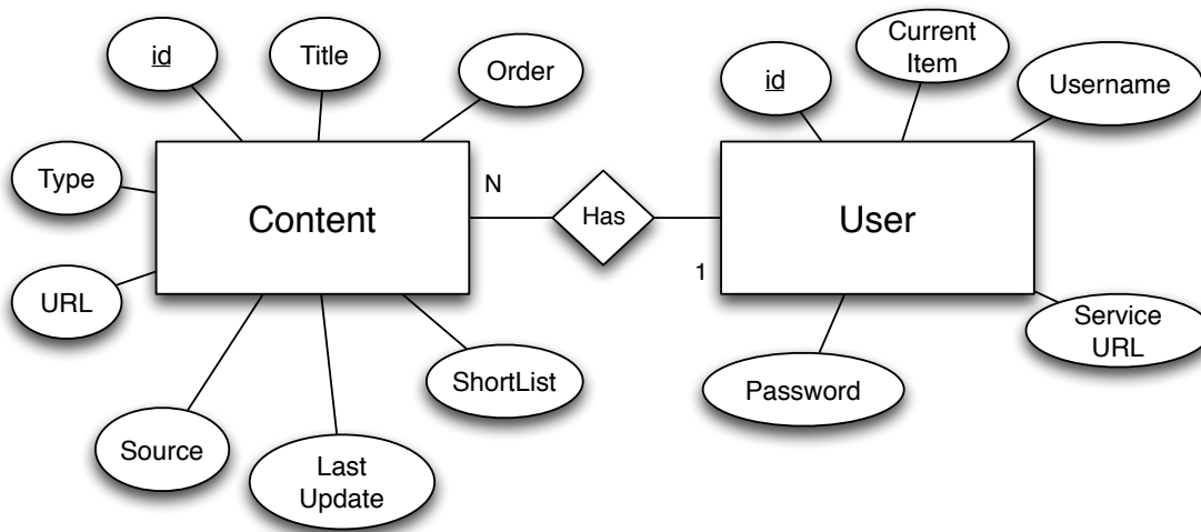
Figure 4.10: The iiD database.
