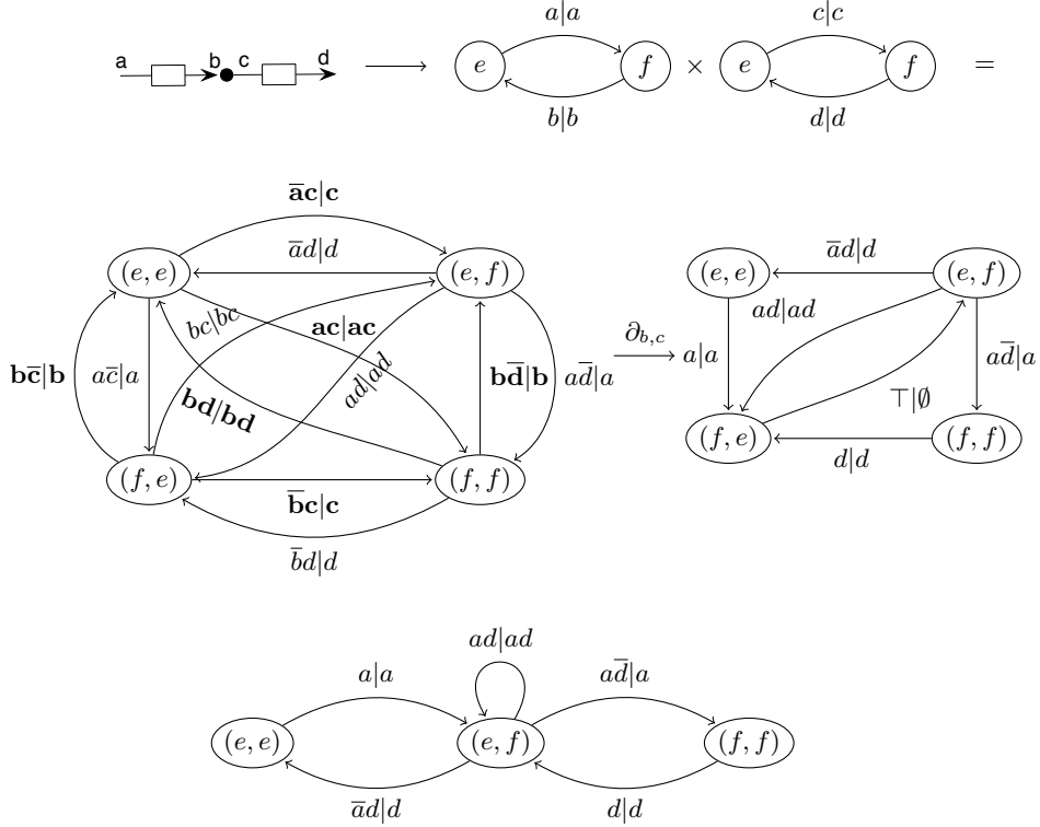
Figure 6: Two FIFO0 buffers plugged together, their automaton, and the result of performing ‘hiding’—a FIFO1 buffer.
