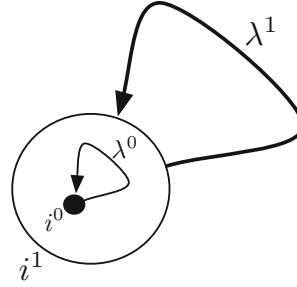
Fig. 2. \mathcal{H}^2TRIV -model
