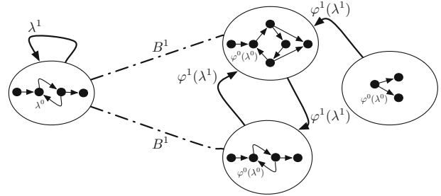
Fig. 8. \mathcal{H}^2 TRIV-Bisimulation
