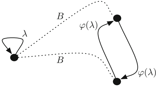
Fig. 5. \mathcal{H}TRIV -Bisimulation
