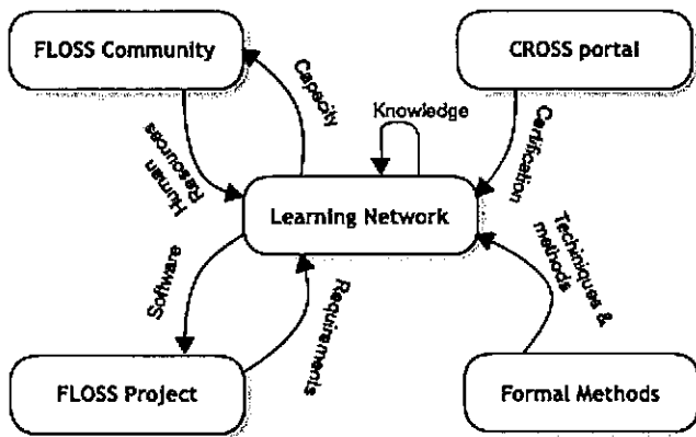
Fig. 1. The problem domain.
