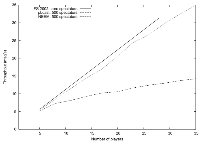
Fig. 5. FS2002 performance.
