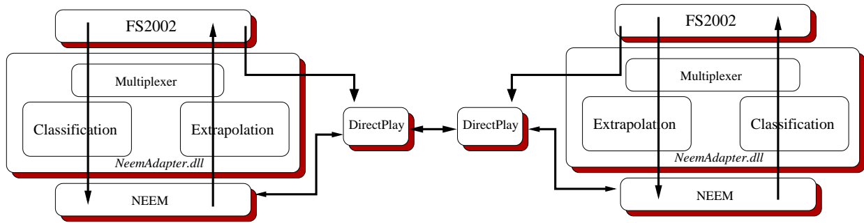
Fig. 3. Integration architecture.
