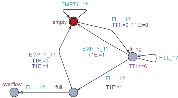
Fig. 4. UPPAAL model of the tank1.
