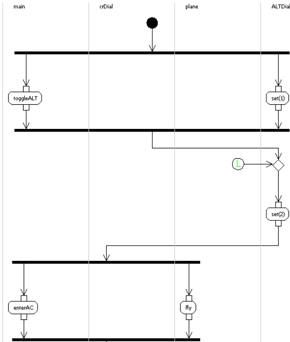
(c) Activity diagram representation
