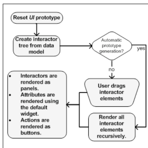
Figure 5. User Interface Mapping and Generation
