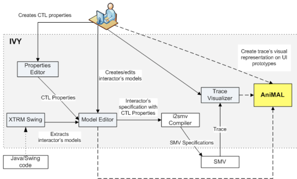
Figure 1. IVY workbench workflow
