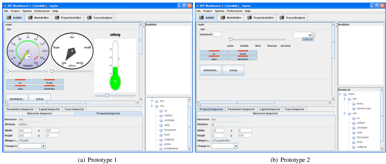
Figure 8. Two customised user interface prototypes
