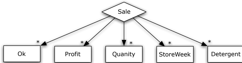
Figure 3.6: Optimized RID graph for our running example.
