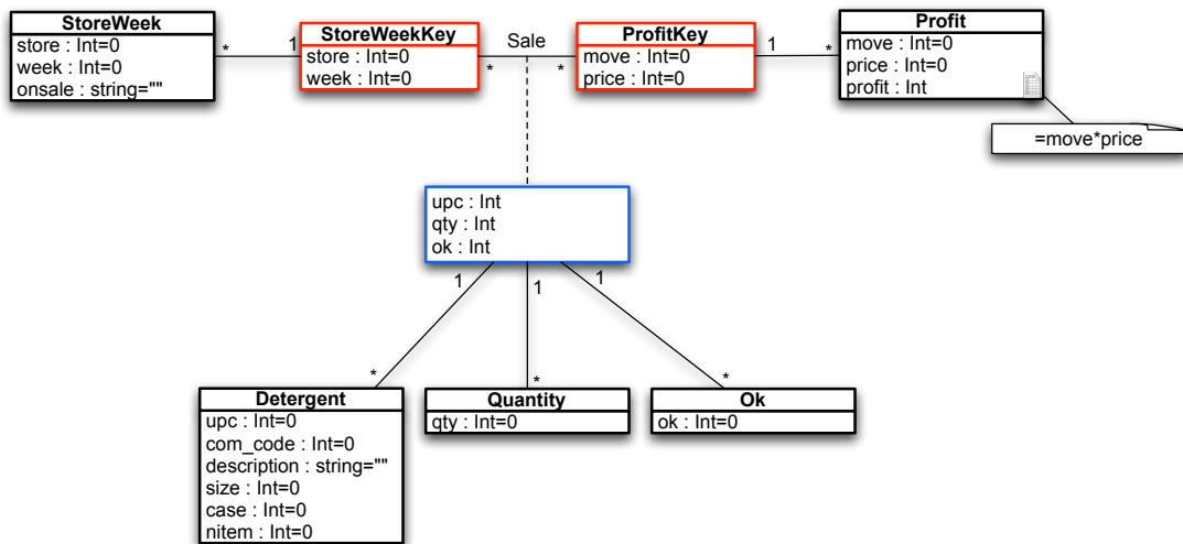
Figure 3.3: A class diagram specifying the sales system for dishwasher detergents.
